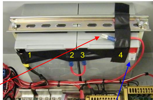
Fig 1-2 Battery Installation
