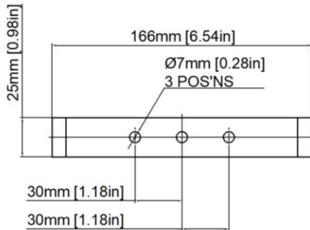
Figure 2: Fixing Location for GNEXS2[F/H] Sounder.
