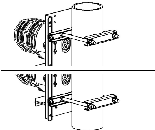
Fig. 2: Pole Mounted Unit Max. Pole size NPS 4" (OD: Ø114.3mm / 4.5in)
