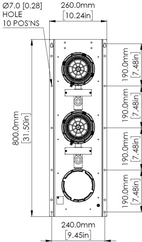
Fig. 1: Mounting Detail and Dimensions for D1x Status Light
