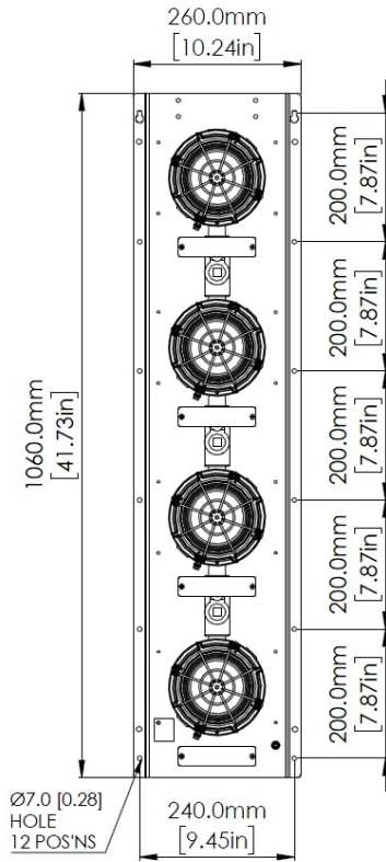
Fig.1: Mounting Detail and Dimensions for D1x Status Light
