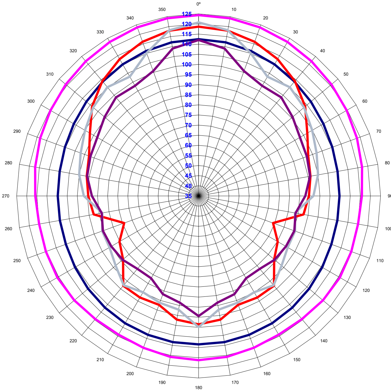
D2xL2F Loudspeaker Polar Plot
