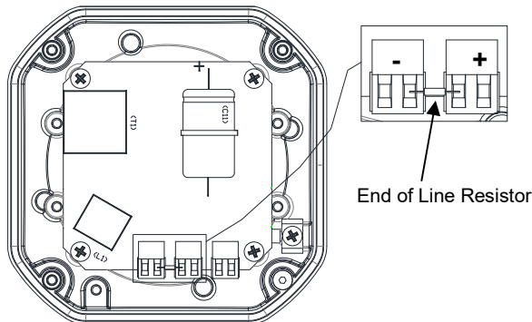
Fig. 7 End of Line Resistor Forming
