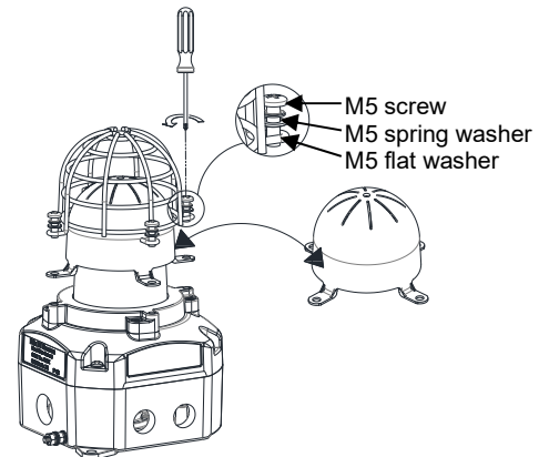
Fig. 9 Replacement of beacon lens cover
