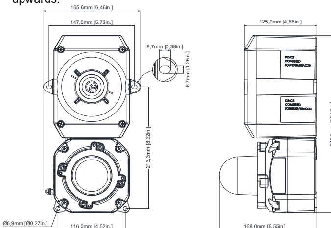
Fig. 1 Fixing locations.
