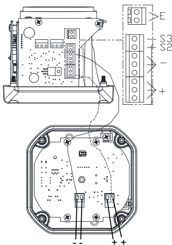
Fig. 4 Terminals
