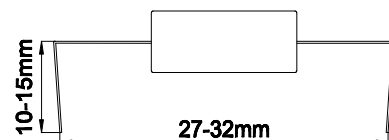
Fig. 6a End of Line Resistor Forming
