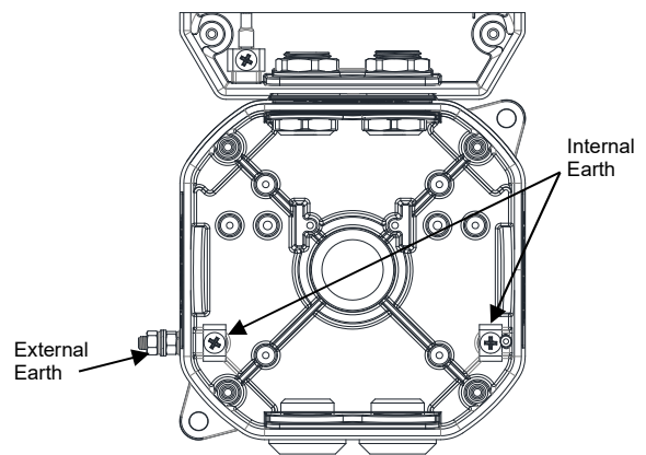
Fig. 5 Earth locations
