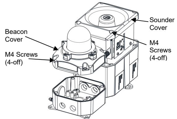
Fig. 2 Accessing the Enclosures.
