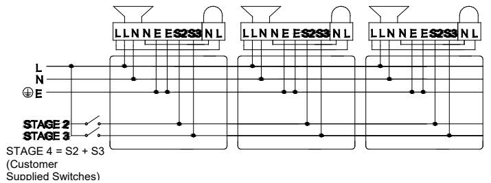
Fig 5b. D1xC1 AC Simplified Block Diagram
