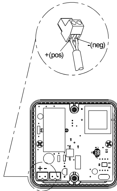
AL100XDC024 Beacon PCBA 20-28 VDC
