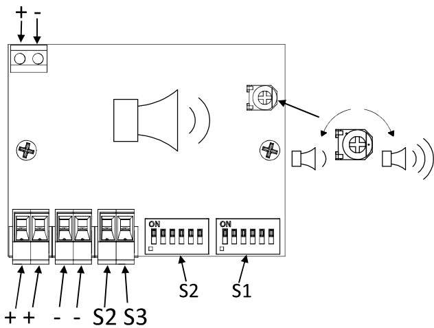
AL100XDC024 Sounder PCBA
