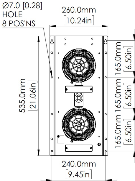
Fig.1: Mounting Detail and Dimensions for D1x Status Light
