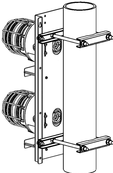
Fig. 2: Pole Mounted Stack Max. Pole size NPS 4" (OD: Ø114.3mm / 4.5in)
