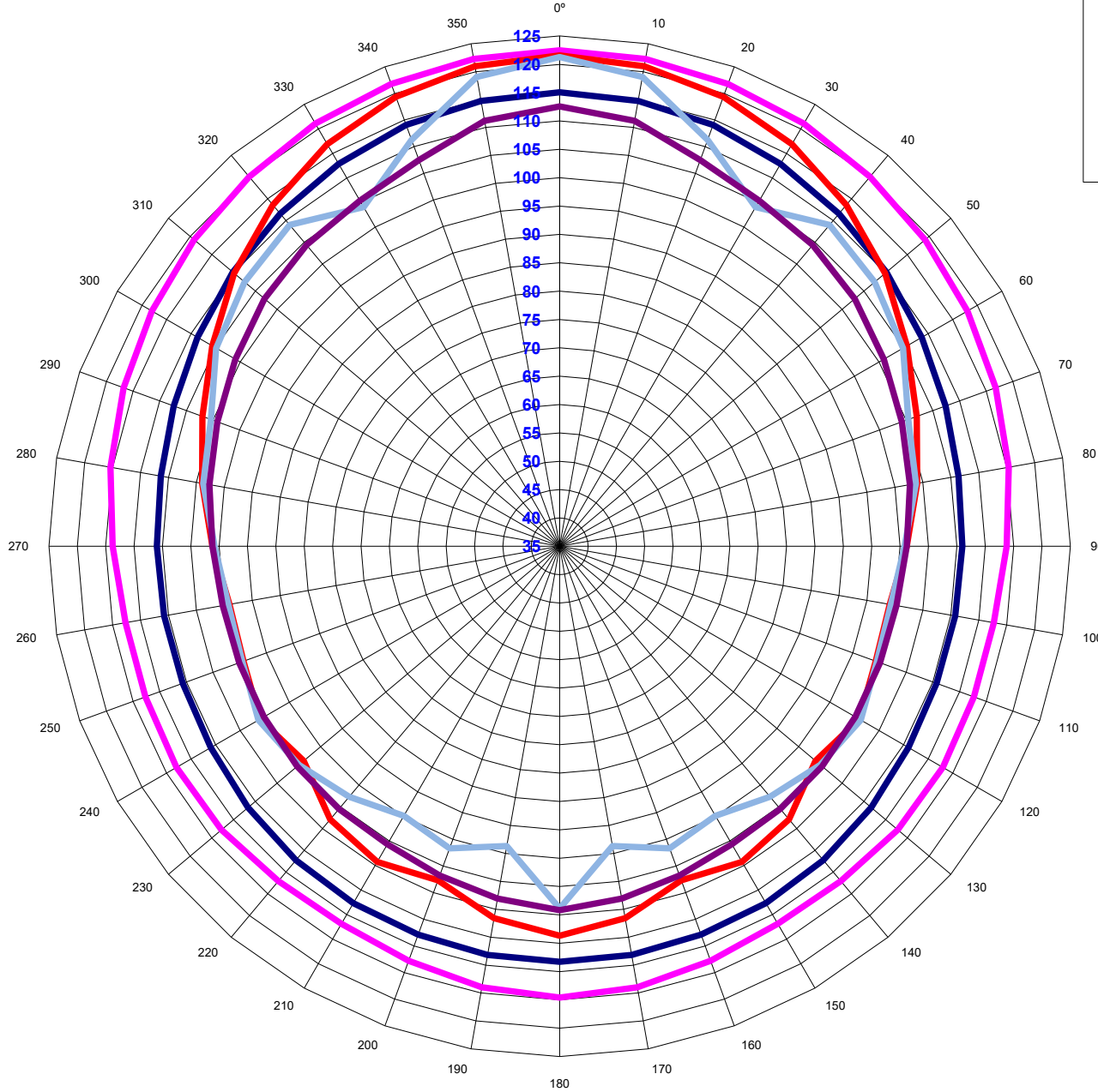
ML25F Loudspeaker Polar Plot
