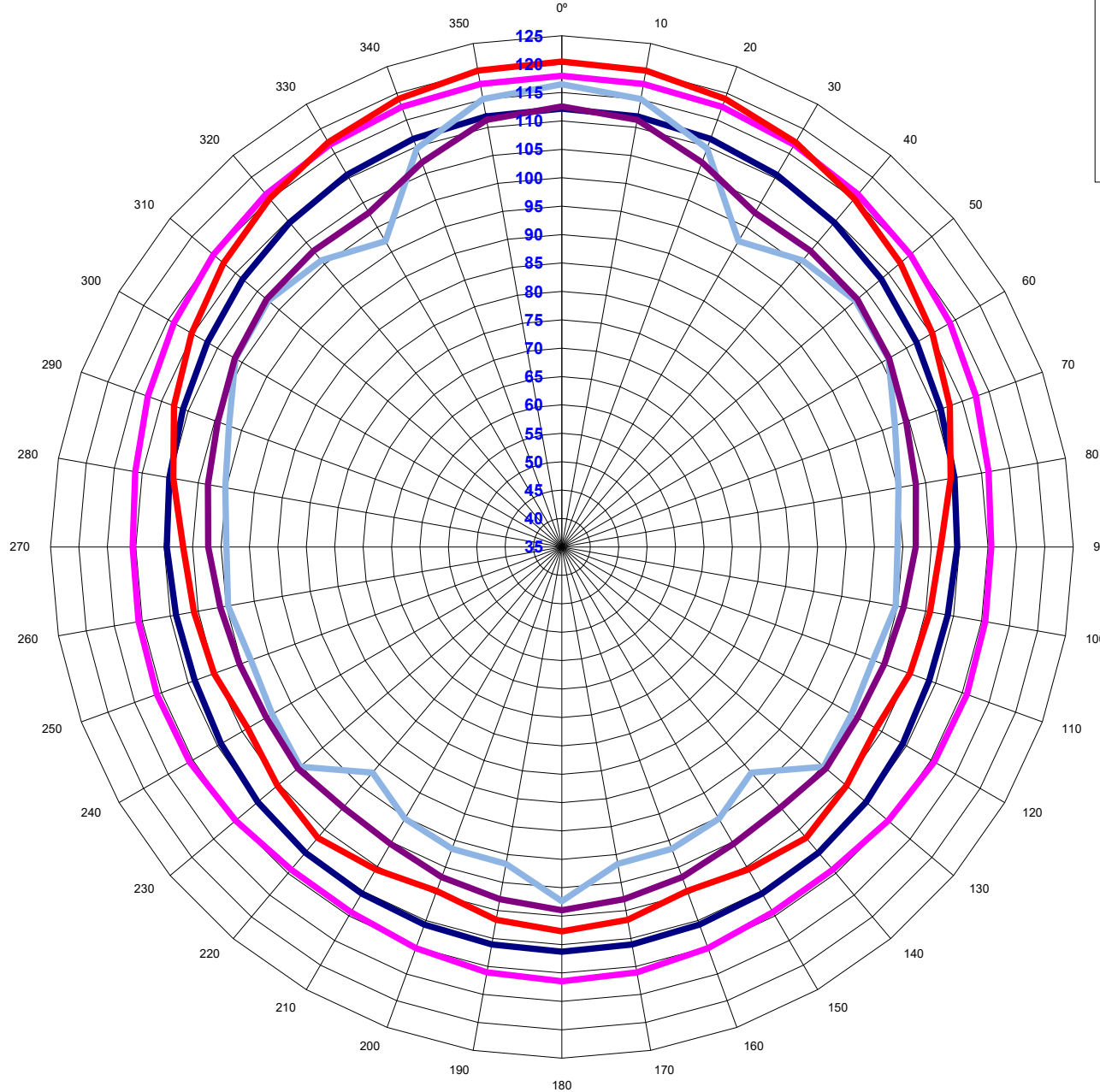
ML15F Loudspeaker Polar Plot
