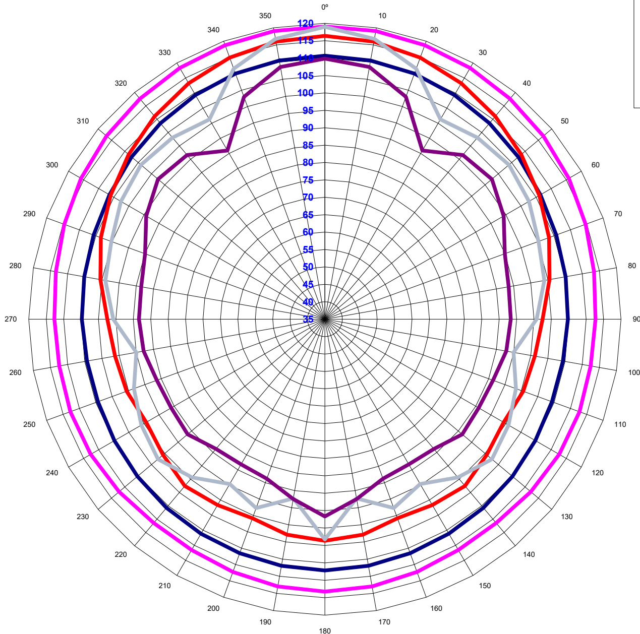
D2xL1F Loudspeaker Polar Plot
