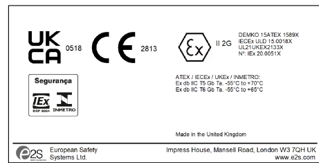
STExCP8-PM-S-L (WITH MODULE) PRODUCT LABEL 2
