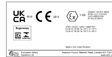
STExCP8-PT-S-C (WITH MODULE) PRODUCT LABEL 2
