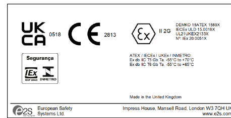
STExCP8-PB-S-L (WITH MODULE) PRODUCT LABEL 2
