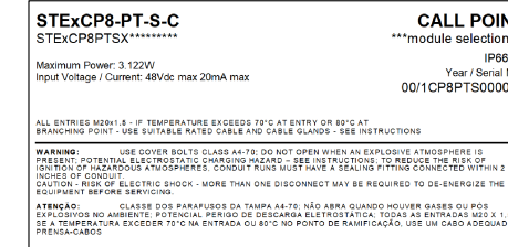
STExCP8-PT-S-C (WITH MODULE) PRODUCT LABEL 1
