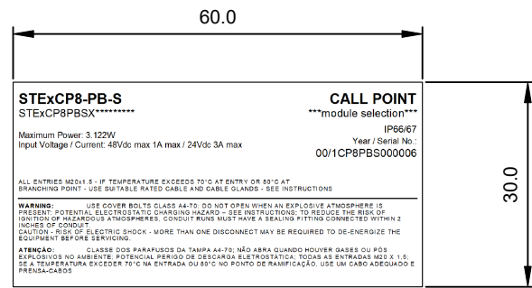
STExCP8-PB-S (WITH MODULE) PRODUCT LABEL 1
