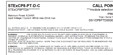
STExCP8-PT-D-C (WITH MODULE) PRODUCT LABEL 1
