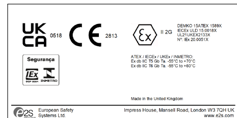
STExCP8-PT-D (WITH MODULE) PRODUCT LABEL 2
