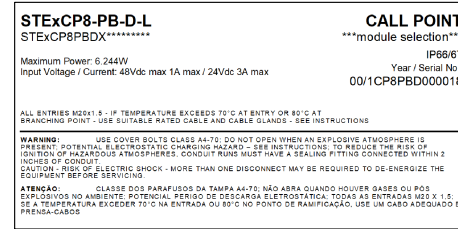
STExCP8-PB-D-L (WITH MODULE) PRODUCT LABEL 1
