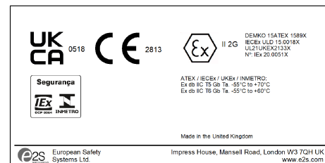
STExCP8-PB-D (WITH MODULE) PRODUCT LABEL 2
