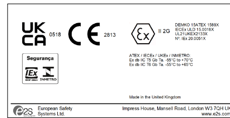
STExCP8-PT-S-L (WITH MODULE) PRODUCT LABEL 2
