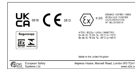
STExCP8-PB-S-C (WITH MODULE) PRODUCT LABEL 2
