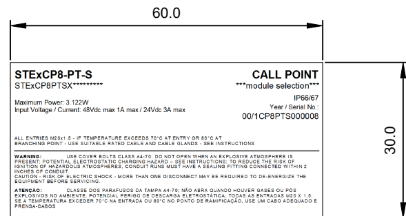
STExCP8-PT-S (WITH MODULE) PRODUCT LABEL 1
