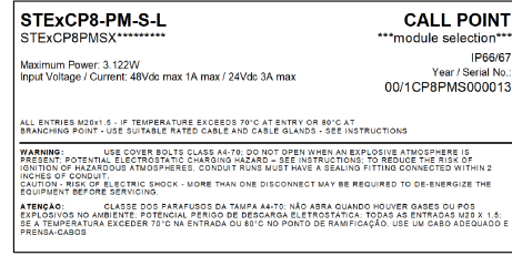
STExCP8-PM-S-L (WITH MODULE) PRODUCT LABEL 1
