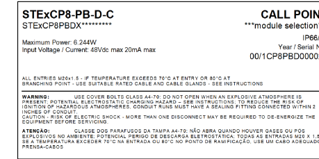
STExCP8-PB-D-C (WITH MODULE) PRODUCT LABEL 1
