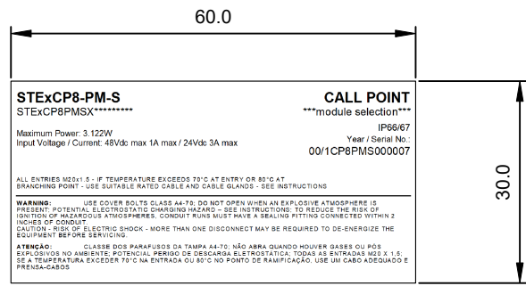
STExCP8-PM-S (WITH MODULE) PRODUCT LABEL 1
