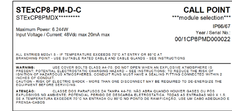
STExCP8-PM-D-C (WITH MODULE) PRODUCT LABEL 1
