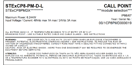
STExCP8-PM-D-L (WITH MODULE) PRODUCT LABEL 1
