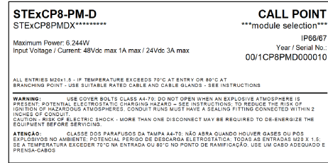
STExCP8-PM-D (WITH MODULE) PRODUCT LABEL 1
