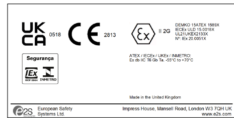
STExCP8-PT-S (WITH MODULE) PRODUCT LABEL 2
