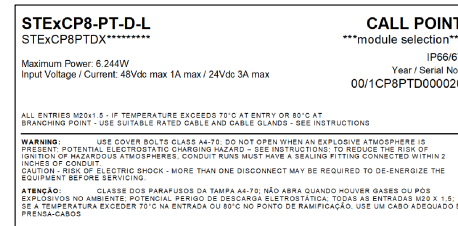
STExCP8-PT-D-L (WITH MODULE) PRODUCT LABEL 1
