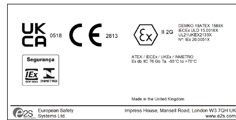
STExCP8-PB-S (WITH MODULE) PRODUCT LABEL 2
