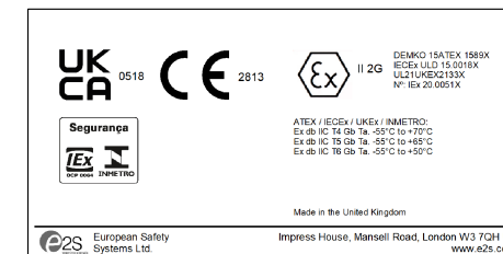
STExCP8-PB-D-C (WITH MODULE) PRODUCT LABEL 2
