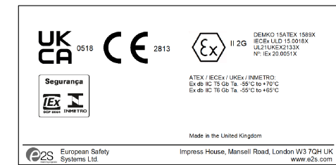
STExCP8-PM-S-C (WITH MODULE) PRODUCT LABEL 2
