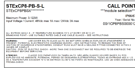
STExCP8-PB-S-L (WITH MODULE) PRODUCT LABEL 1
