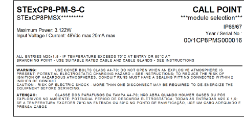
STExCP8-PM-S-C (WITH MODULE) PRODUCT LABEL 1
