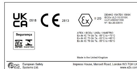
STExCP8-PT-D-L (WITH MODULE) PRODUCT LABEL 2
