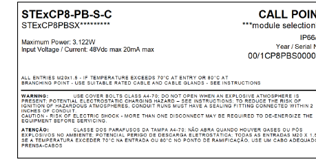
STExCP8-PB-S-C (WITH MODULE) PRODUCT LABEL 1
