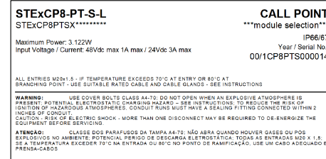
STExCP8-PT-S-L (WITH MODULE) PRODUCT LABEL 1
