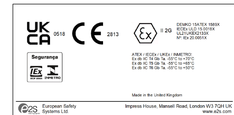
STExCP8-PM-D-C (WITH MODULE) PRODUCT LABEL 2
