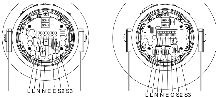
D1xS1AC Terminals
