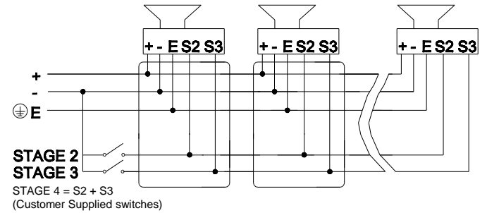
Fig. 7a DC Simplified Block Diagram (negative switching)
