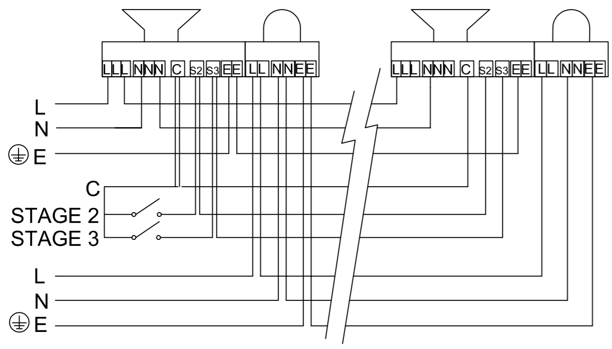
AC - INDEPENDENTLY POWERED SOUNDER & BEACON
