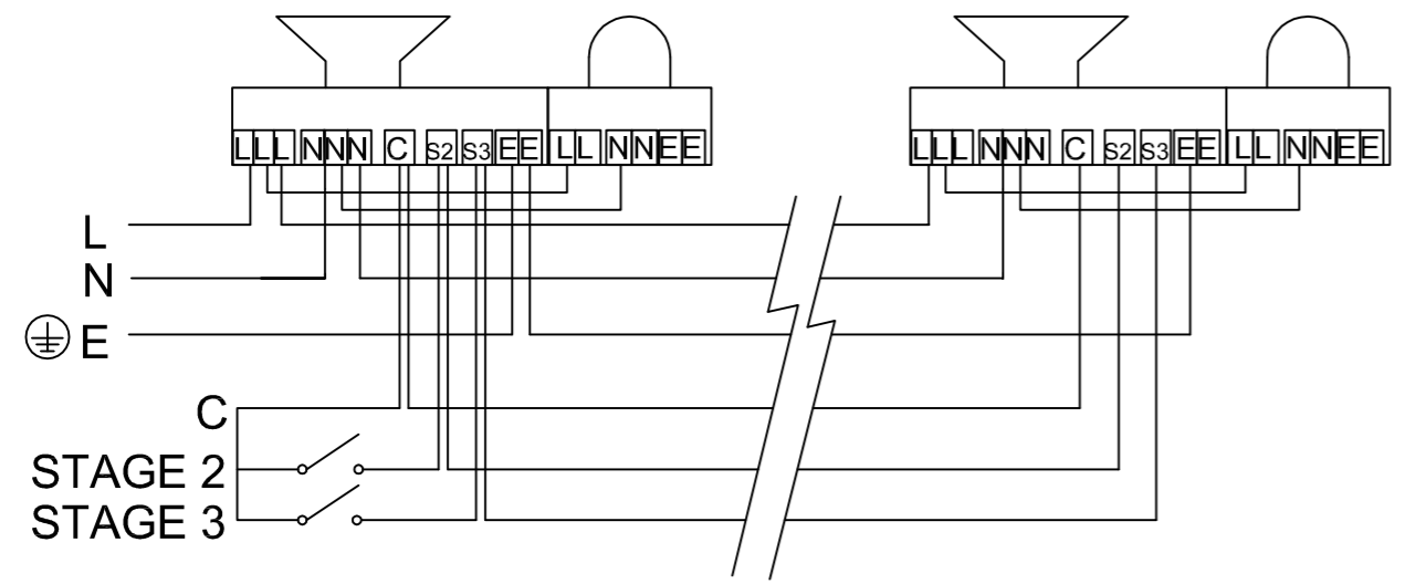
AC - SIMULTANEOUSLY POWERED SOUNDER & BEACON
