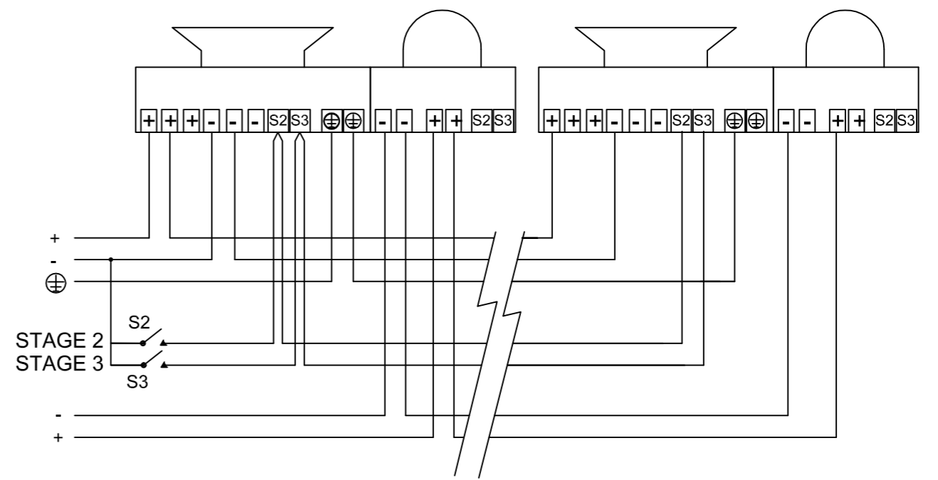
DC - INDEPENDENTLY POWERED SOUNDER & BEACON
