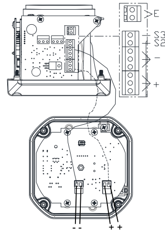
Fig. 4 Terminals
