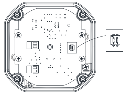
Fig. 9: DIP Switch Location
