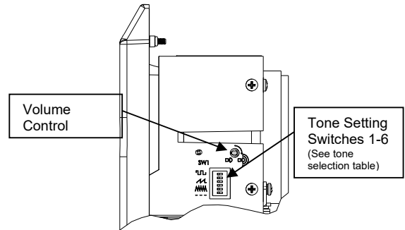
Fig. 8 Location of field controls
