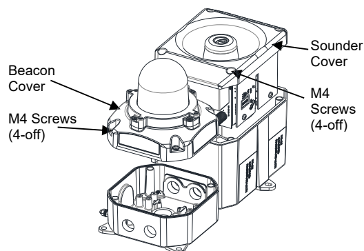
Fig. 2 Accessing the Enclosures.
