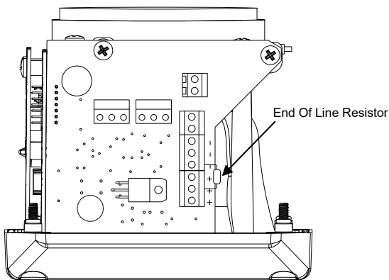
Fig. 7b End of Line Resistor Placement – Sounder
