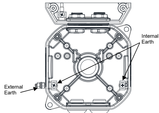
Fig. 5 Earth locations
