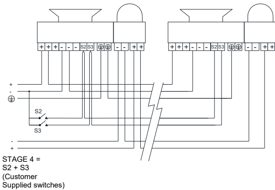
Fig. 3b Simplified Block Diagram Beacon & Sounder Powered Independently
