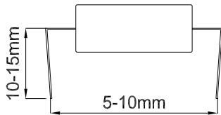
Fig. 7a End of Line Resistor Forming
