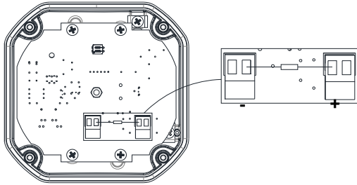
Fig. 6b End of Line Resistor Placement - Beacon
