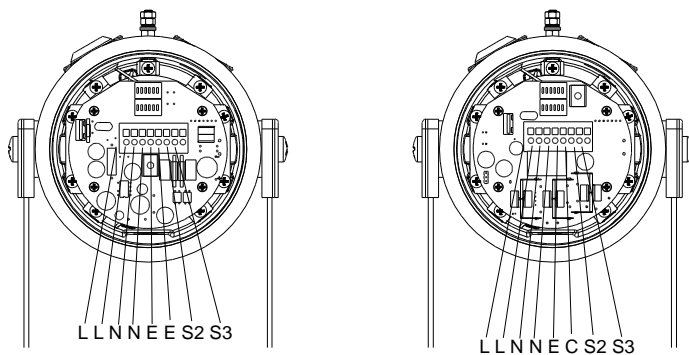
Fig. 6 AC Terminals
