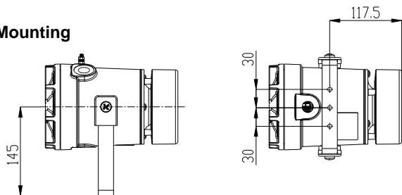
Fig. 1 Fixing locations.
