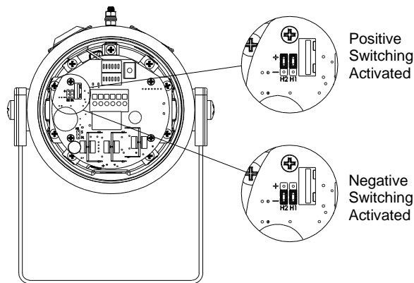
Fig. 4 Stage Switching Polarity
