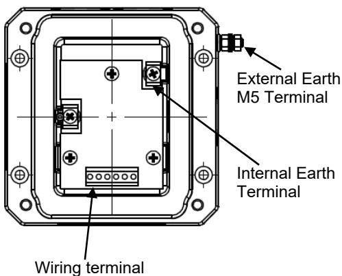
Fig 3 Earth terminals
