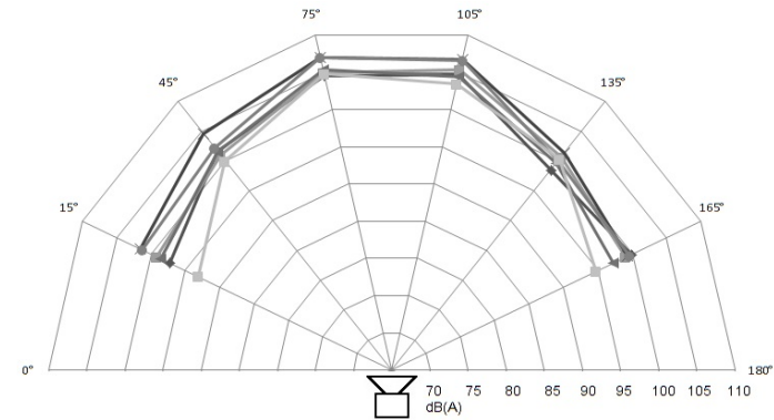
SONFL1XDC024-H VERTICAL POLAR PLOT
