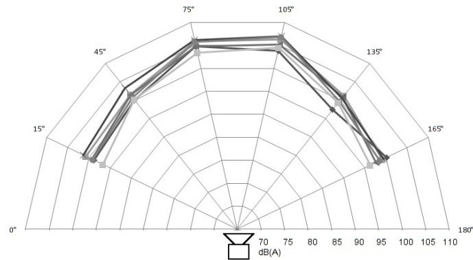
SONFL1XDC024-H HORIZONTAL POLAR PLOT
