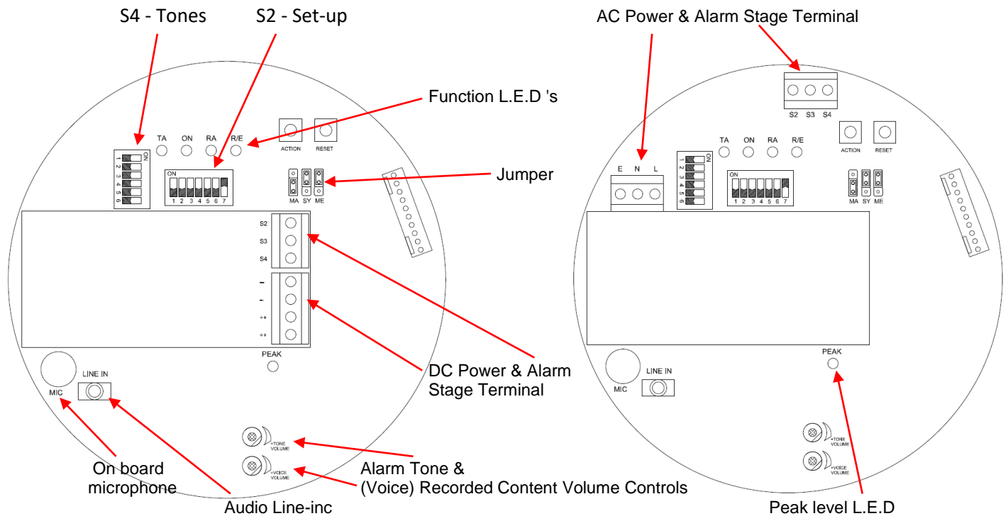
DC A121AX, MV121, AL121AXH & AL121AXX Board
