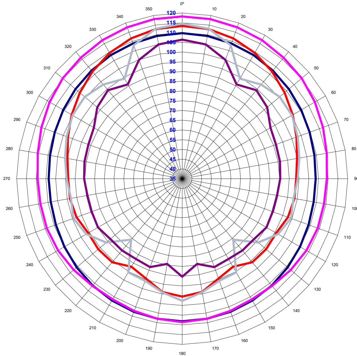
D1xL1F Loudspeaker Polar Plot
