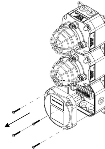
Fig. 2: Accessing the Junction Box Terminals
