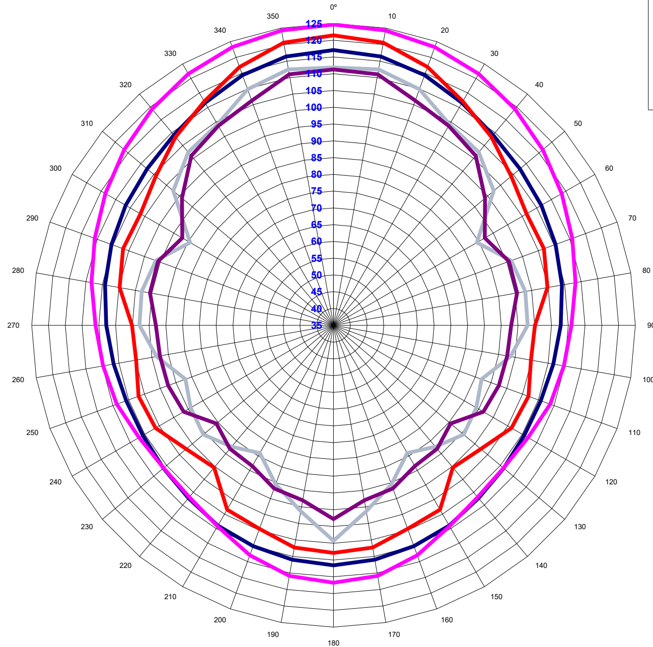
D2xL2H Loudspeaker Polar Plot
