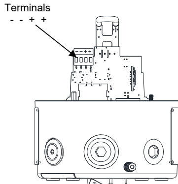
Fig. 3 D1xB2XDC Terminals
