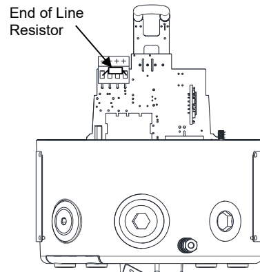
Fig. 5b End of Line Resistor Placement
