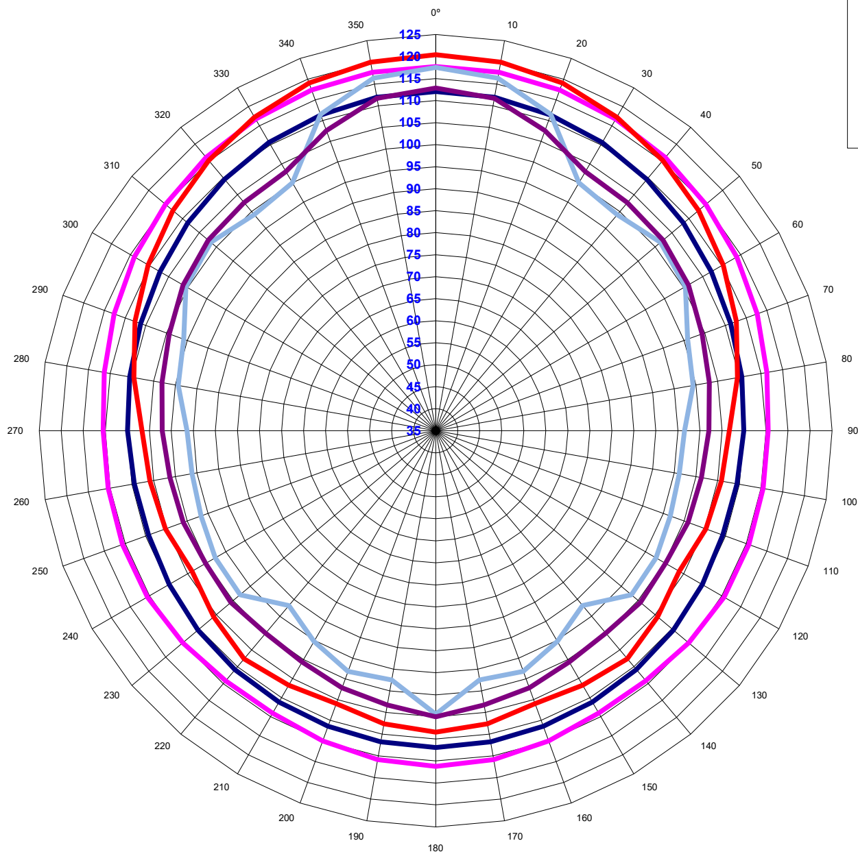
E2xL15F Loudspeaker Polar Plot
