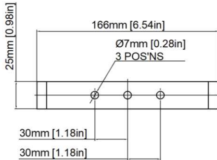
Figure 2: Fixing Location for GNEsS1[F/R] Sounder.
