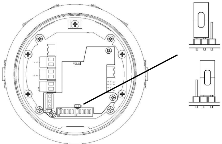
Figure 16: J2 Header pin positions – Fault Resistor (FR)
