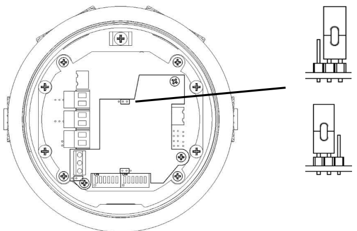
Figure 17: J3 Header pin positions – Hard Reset Function
