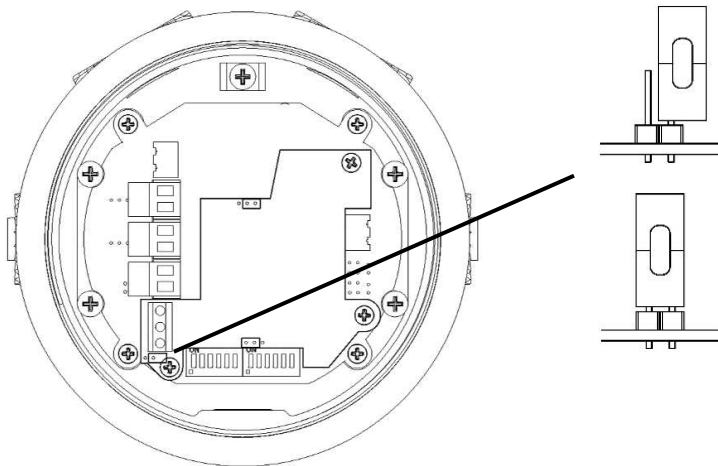
Figure 15: J1 Header pin positions – Current Sense Resistor (CSR)
