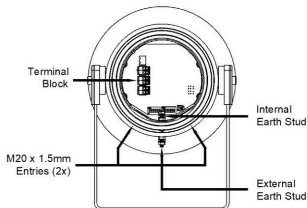
Figure 5: GNEExS1 Entries and Terminal Block Location.
