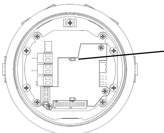
Figure 18: J3 Header pin positions – Hard Reset Function
