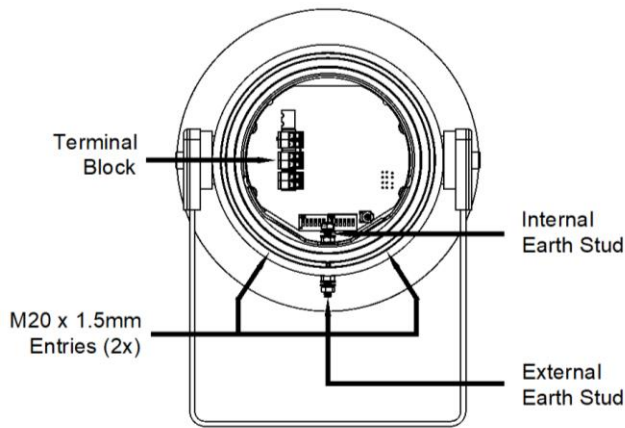
Figure 6: GNEsS2 Entries and Terminal Block Location.
