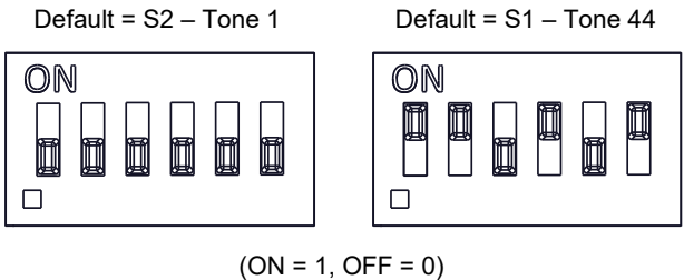
Figure 10: DIP switch configuration
