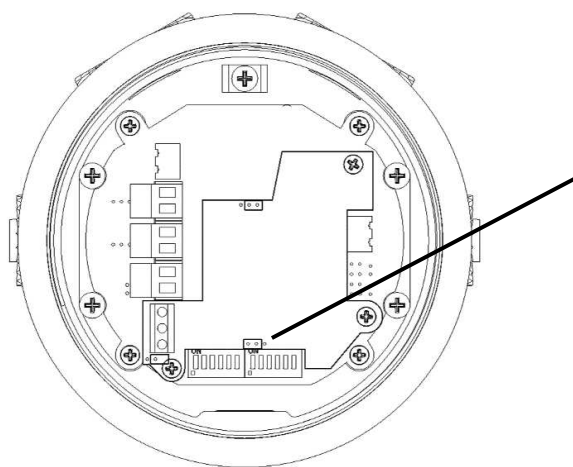
Figure 17: J2 Header pin positions – Fault Resistor (FR)
