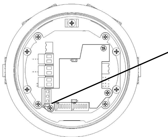
Figure 16: J1 Header pin positions – Current Sense Resistor (CSR)
