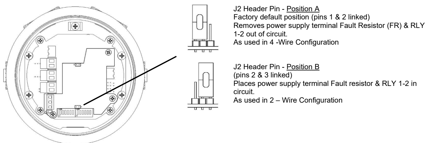
Figure 12: J2 Header pin positions – Fault Resistor (FR)
