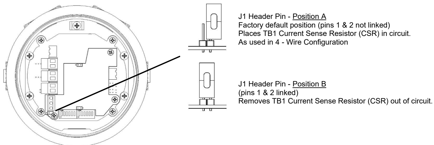
Figure 11: J1 Header pin positions – Current Sense Resistor (CSR)
