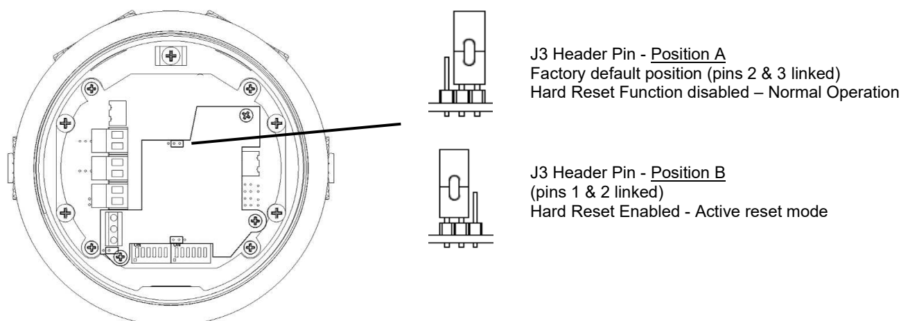
Figure 13: J3 Header pin positions – Hard Reset Function
