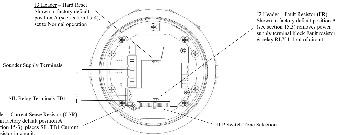
Figure 10 – Terminals and header pins for sounder
