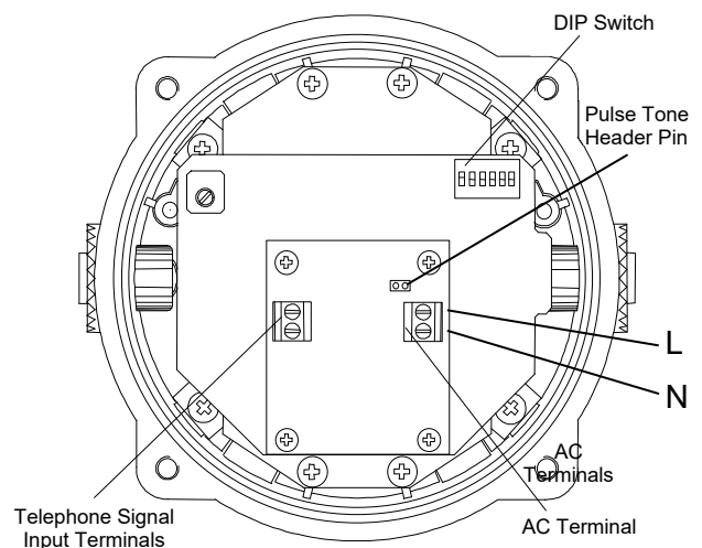
Fig. 4 AC Terminals
