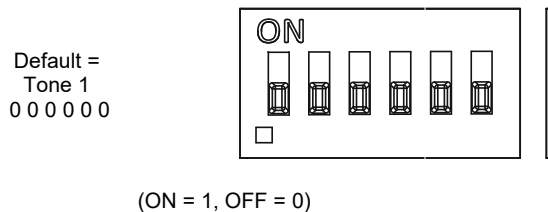
Figure 9: DIP switch configuration
