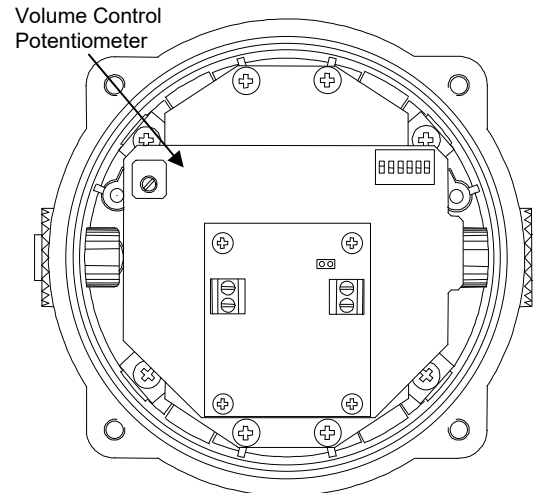
Location of Volume Control Potentiometer
