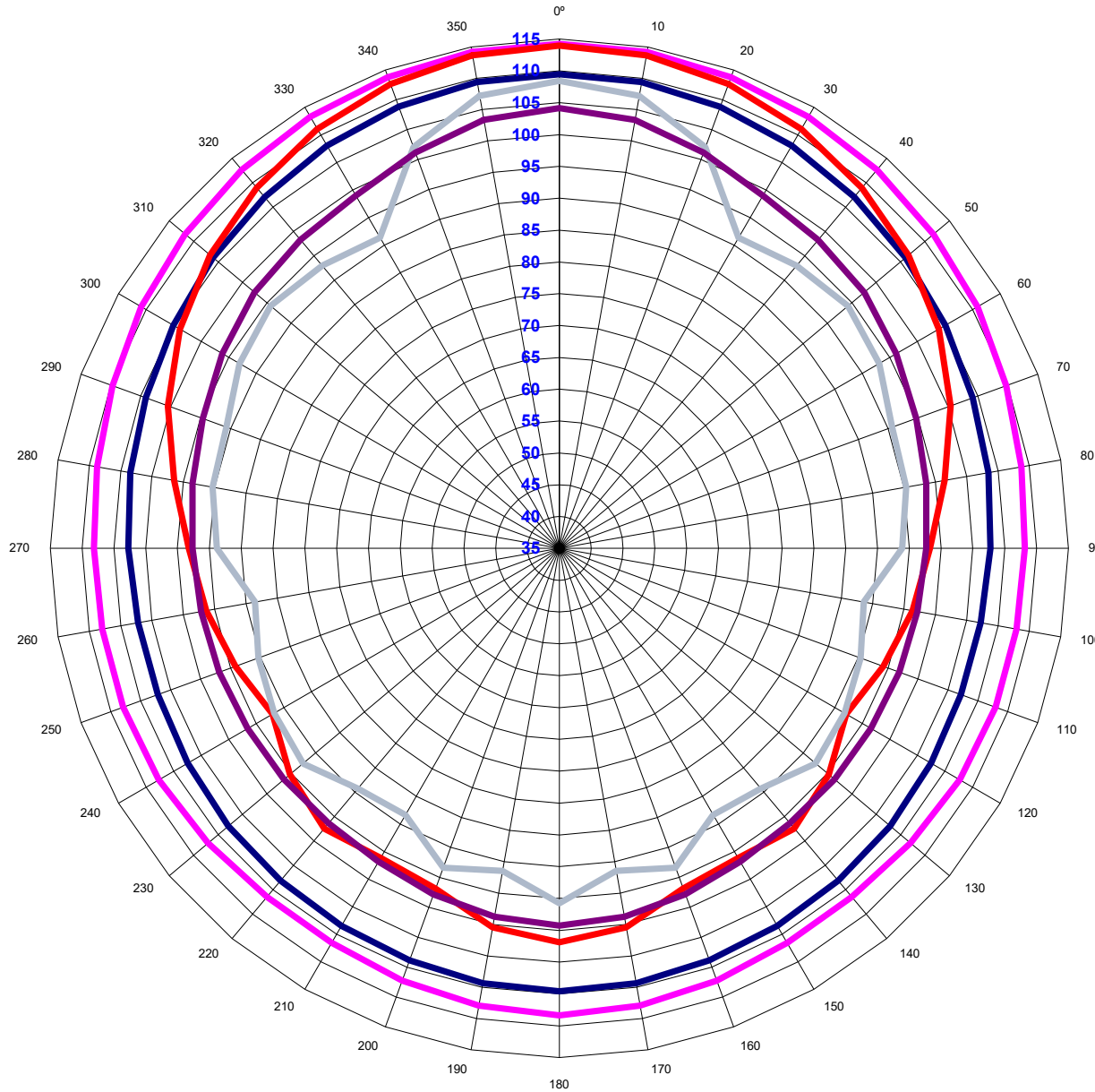
STExL1F Loudspeaker Polar Plot
