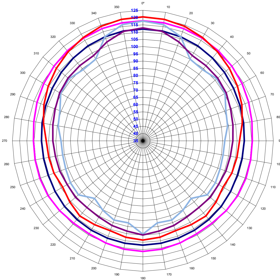
E2xL15F Loudspeaker Polar Plot
