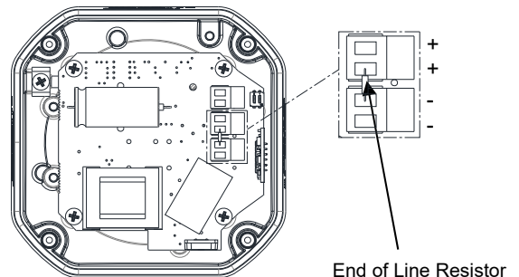
Fig. 6a End of Line Resistor Placement - Beacon
