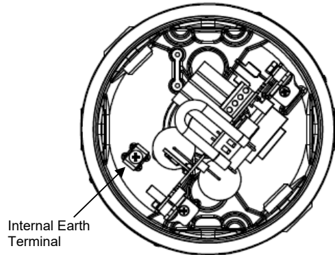
Fig. 5: Internal Earth Location
