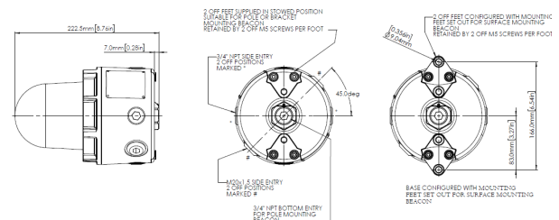
Fig. 1 Fixing Location for Public Mode Beacon
