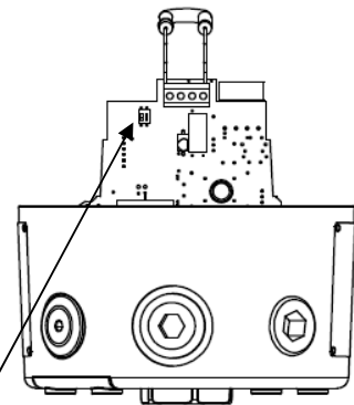
Fig. 6a: DIP Switch Location
