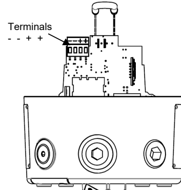
Fig. 3 D1xB2XH1 Terminals
