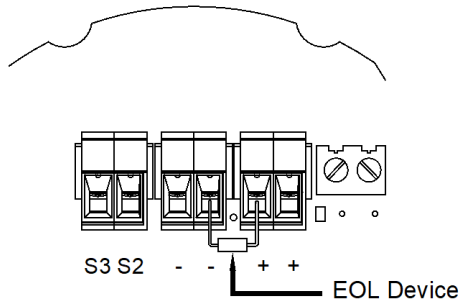
Figure 10: End of Line Resistor placement.
