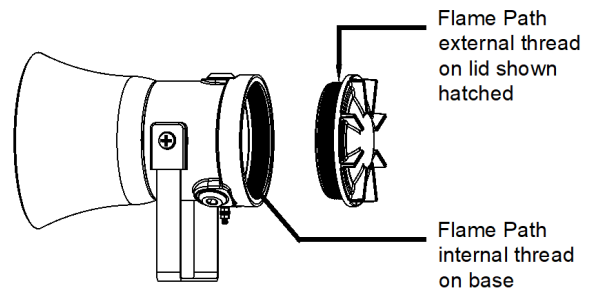
Figure 1: Flame Path
