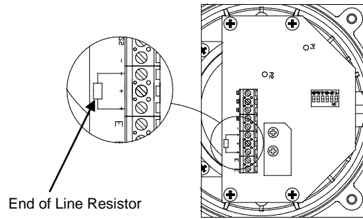
Fig. 8 End of Line Resistor Placement on Sounder
