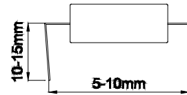
Fig. 9a End of Line Resistor Forming
