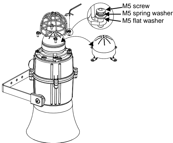
Fig. 10 Replacement of beacon lens cover
